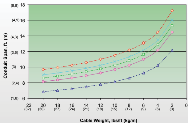
2" (53 mm) XHW Conduit (ID only)
