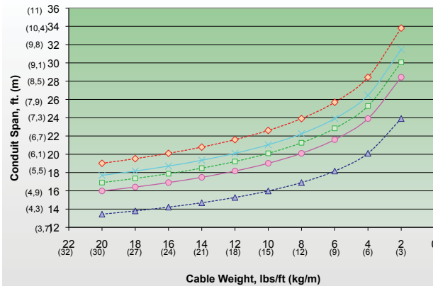
6" (203 mm) XHW Conduit (ID only)
