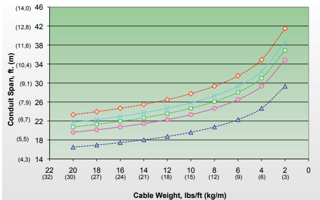
8" (203 mm) XHW Conduit (IPS only)
