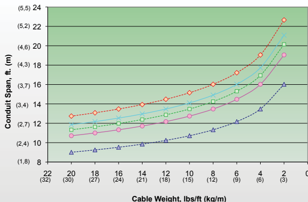
3" (78 mm) XHW Conduit (ID only)
