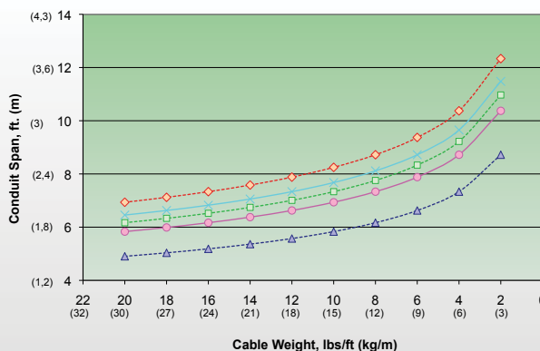
1" (27 mm) XHW Conduit (IPS only)
